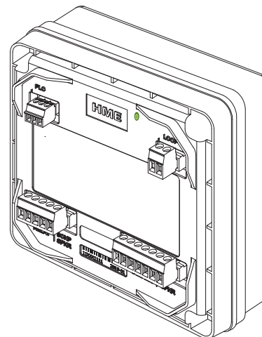
Fig. 2 Connector Side
